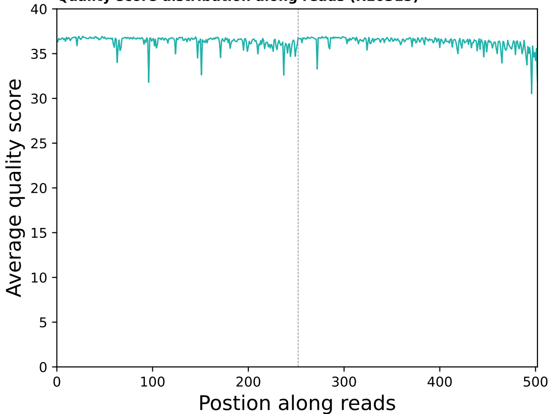
Quality score distribution along reads (R10315)
